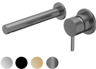
Anthem Wall Mounted Basin Mixer (waste not included) Minimum recommended pressure 0.2bar 160(w) x 120(h) x 180(d)mm
